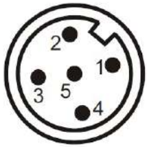
M12x1 5針
