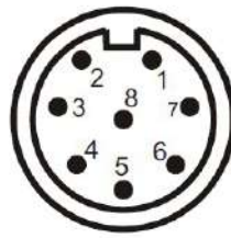
M12x1 8針
